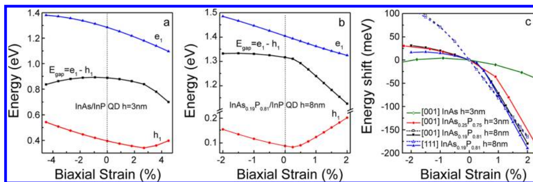
Figure 5. Evolution of the ground electron ( e_1 ) and hole ( h_1 ) energies and the single particle gap ( E_{\text{gap}} = e_1 - h_1 ) as a function of externally applied (lateral) biaxial strain for (a) InAs/InP NW-QD of 3 nm height and (b) alloyed InAs 0.19 P 0.81 NW-QD of 8 nm. (c) Relative energy shift compared to the unstrained system for different QD configurations. Positive values correspond to tensile biaxial strain, while negative values correspond to compressive biaxial strain. The dotted lines correspond to the pseudomorphic cylinder external strain model.
