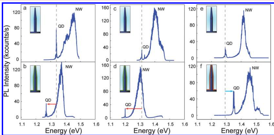
Figure 4. By changing the deposition conditions of the SiO 2 envelope, the energy of the band gap can be tuned: (a) PL of the NW before SiO 2 deposition, (b) PL of the same NW as in (a) with a SiO 2 envelope deposited with increased silane flow. The PL is red-shifted for the NW with 52 meV and for the QD with 45 meV. (c) PL of the NW before SiO 2 deposition and (d) same NW as in (c) with a SiO 2 envelope deposited with increased RF power. The PL is red-shifted for the NW over 110 and 116 meV for the QD. (e) PL before SiO 2 deposition and (f) same NW as in (e) with a SiO 2 envelope deposited with TEOS-PECVD. The PL is now blue-shifted over 55 meV for the QD and 35 meV for the NW.
