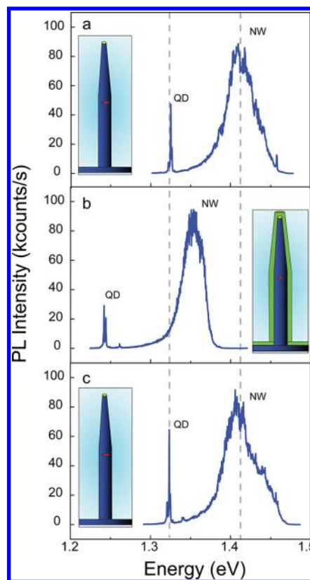
Figure 2. (a) Photoluminescence (PL) of an as-grown InP NW with an InAsP QD, (b) same NW as in (a), but now with a SiO 2 envelope. The PL is red-shifted over 59 meV for the NW and 83 meV for the QD. In (c), the SiO 2 envelope is removed, and the PL for the same NW as in (a) and (b) shifts back to its original energy.
