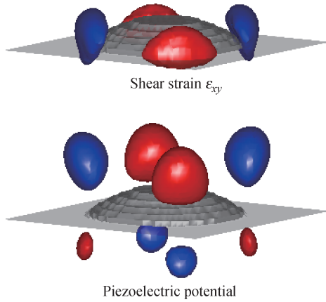
Fig. 2 Isosurface plots of the shear strain component \varepsilon_{xy} and piezoelectric potential in a lens-shaped InAs/GaAs self-assembled quantum dot.
