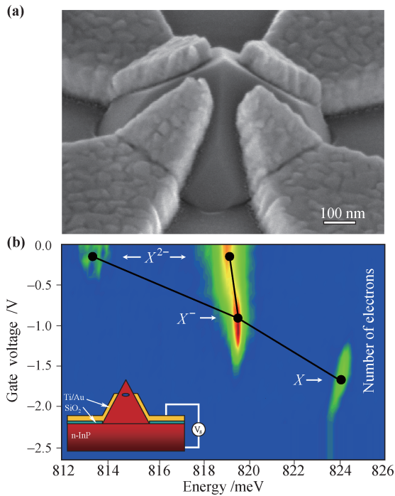
Fig. 14 (a) Single InAs quantum dot in an InP pyramid with metallic gates on the sides of the pyramid. (b) Emission spectrum as a function of the bottom gate voltage. Different emission lines correspond to different charged exciton states, X^0 , X^- , X^{2-} , or different number of electrons in the initial states (right-hand axis). The black circles and lines create a phase diagram of the emission spectrum as predicted in Ref. [27]. Reproduced from Ref. [116], Copyright © 2009 Institute of Physics.
