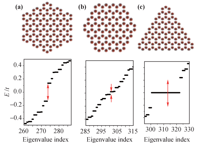
Fig. 18 Single-particle tight-binding spectrum of (a) armchair hexagonal, (b) zigzag hexagonal, and (c) zigzag triangular graphene quantum dot structures consisting of similar number of carbon atoms. Top panel shows the atomic positions. Reproduced from Ref. [133], Copyright © 2010 American Physical Society.
