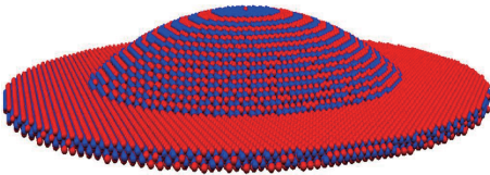
Fig. 1 Indium ( red ) and Arsenic ( blue ) atoms in a lens-shaped InAs quantum dot with diameter of 25 nm and height of 3.5 nm on a 0.6 nm high wetting layer. The GaAs barrier material atoms are not shown.
