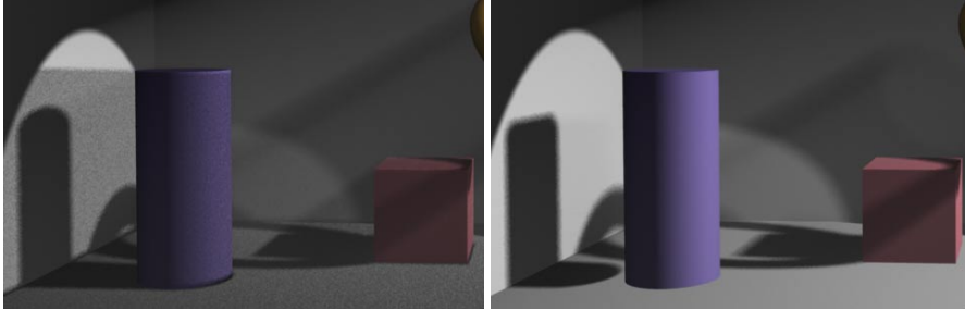
Figure 2.12: Selecting shadow bias. Too small a bias value will result in incorrect self-shadowing (left). Notice the darker, dirtier look compared to Figures 2.11 or 2.10. Too much bias can also introduce artifacts, such as the appearance of “floating objects” or the detached shadow at the bottom of the cylinder (right).
