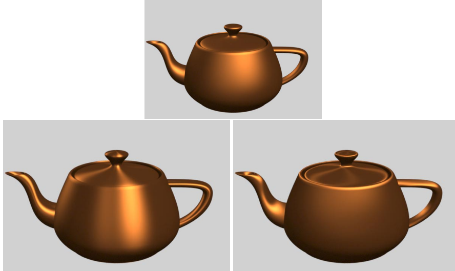
Figure 2.8: Examples of the Ward anisotropic reflection model. Isotropic reflection with xroughness=yroughness=0.3 (top). Anisotropic reflection with xroughness=0.15 , yroughness=0.5 (bottom left). Anisotropic reflection with xroughness=0.5 , yroughness=0.15 (bottom right). In all cases, xdir=normalize(dPdu) .
