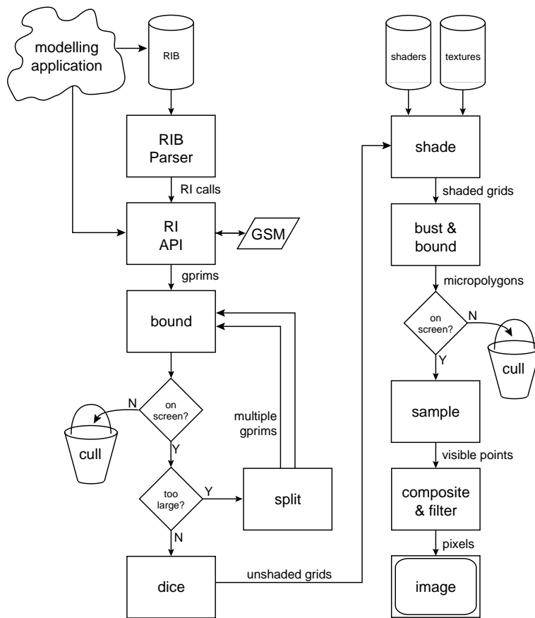
Figure 1.1: The Reyes rendering pipeline.
