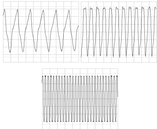
Fig.4. Waveforms of the three modes of an open flute, depending on the „strength” of blowing, from the weakest to the strongest, (OX = 10 ms).
