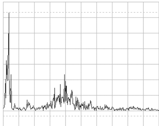
Fig.8b. Frequency spectrum of the big thunder tube obtained by the „virtual oscilloscope” program. [ big4.avi ].
