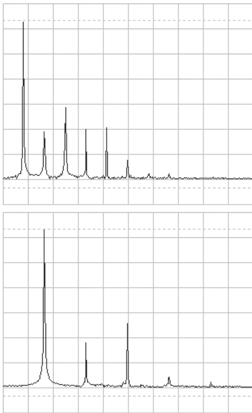
Fig.3a and 3b. Fourier transform analysis of flute spectra - the „weak” and „intermediate blowing”. Two figures differ by the OY scale (a lower amplification factor was applied in fig. 3b), OX scale is the same ( f=0-7046.4 Hz). Note that widening of the lines is not an instrumental effect, as for example for a vibrating glass an almost „Dirac-delta” spectra can be obtained [1].
