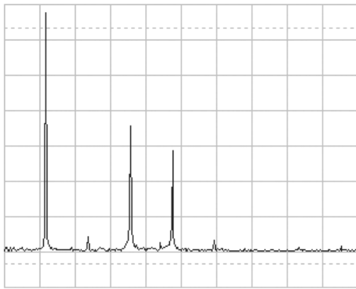
Fig. 6. The lowest mode excited ( \lambda = 3L/4 ) in the closed flute. Note the almost absence of the second harmonics, see also the whole dynamics of the sound on the internet movie file .
