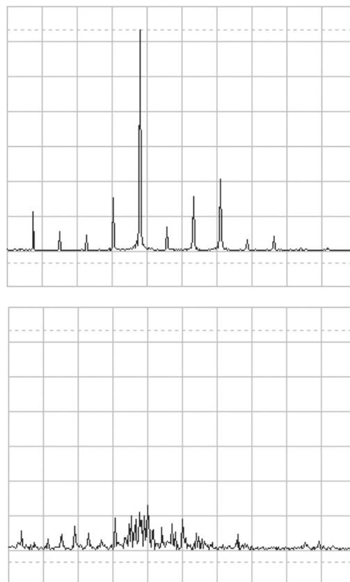
Fig. 12a and 12b. The Fourier transform spectra of a “good” violin – note narrow and perfectly distanced higher harmonics frequencies. The spectrum below has been obtained with the same violin, but with “non-professional” excitation – note the wide peak of “noise” at about 3 kHz.
