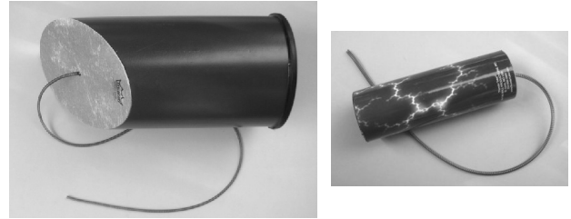
Fig.7. Thunder tubes: tubes open on one side and closed a semi-rigid membrane on the other one, with a flexible spring attached to it. Diameters are 15 cm and 5 cm and lengths 21cm (a shorter border) and 18 cm for the big and small tubes, respectively.
