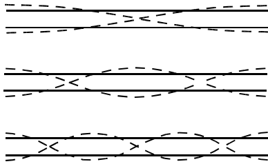
Fig.2. Standing waves modes for a tube opened on both ends: higher harmonics are integer multiplies of the fundamental frequency - 1:2:3 etc.
