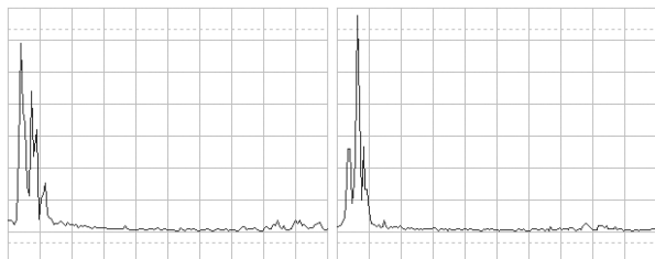
Fig. 10. Reverberation effects on the big thunder tube – intensities of different frequencies fall and grow in time. Single pictures of the presented Fourier-analysis sequence were taken every 0.2 s.
