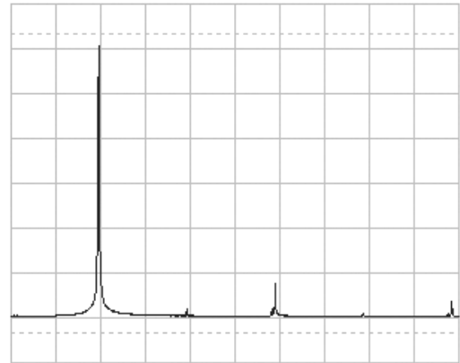
Fig.3c. Fourier transform analysis of flute spectra - the „strongest” blowing for the open flute. Note the doubled OX scale ( f=0-14048.5 Hz) compared to fig. 3a and 3b and an expanded OY scale. Lack of the even frequency multiplies, as on this figure, should be typical for a tube closed on one end, and not open on both ends – it seems that with a high power density of the sound the tube gets capped.
